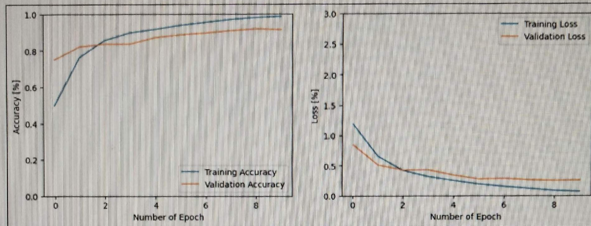
Figure 5. Plot of Evaluation Metrics
